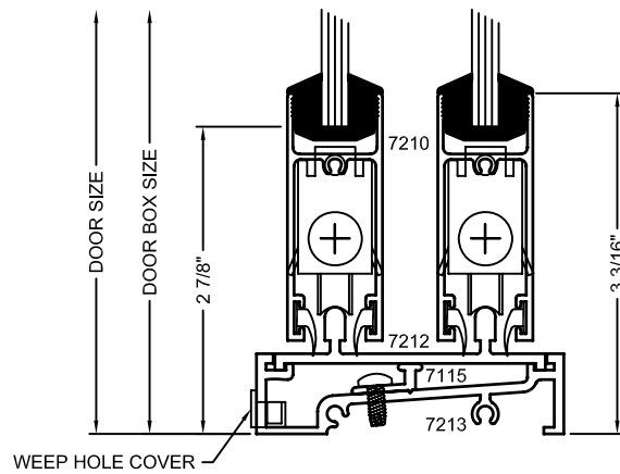
3 SILL DETAIL
