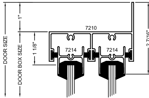
1 HEAD DETAIL
