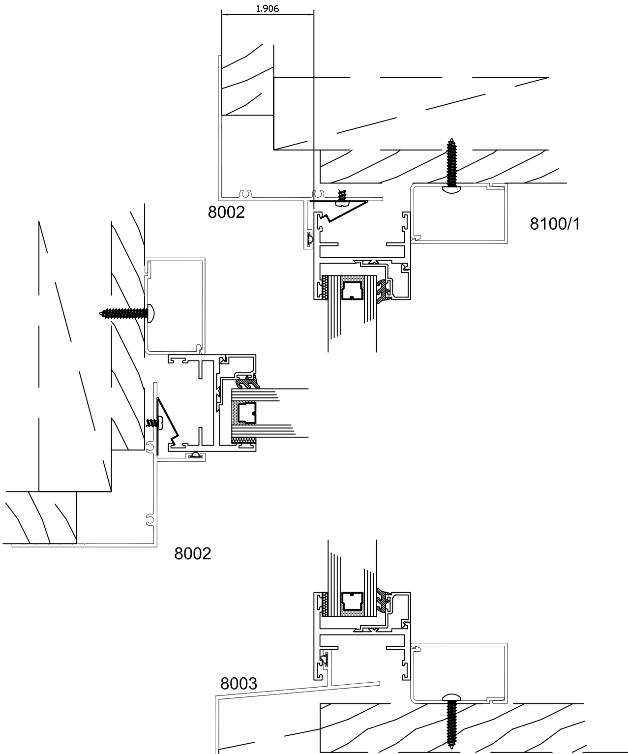
typical 2000 series PANNING installation
