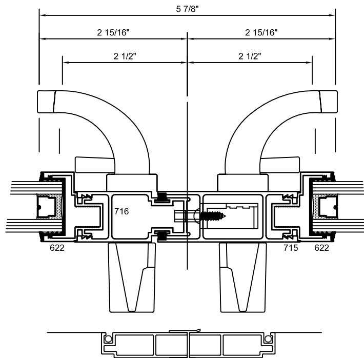
OXO LOCKING RAIL XOO/OOX MEETING RAIL (OMIT HANDLE)
