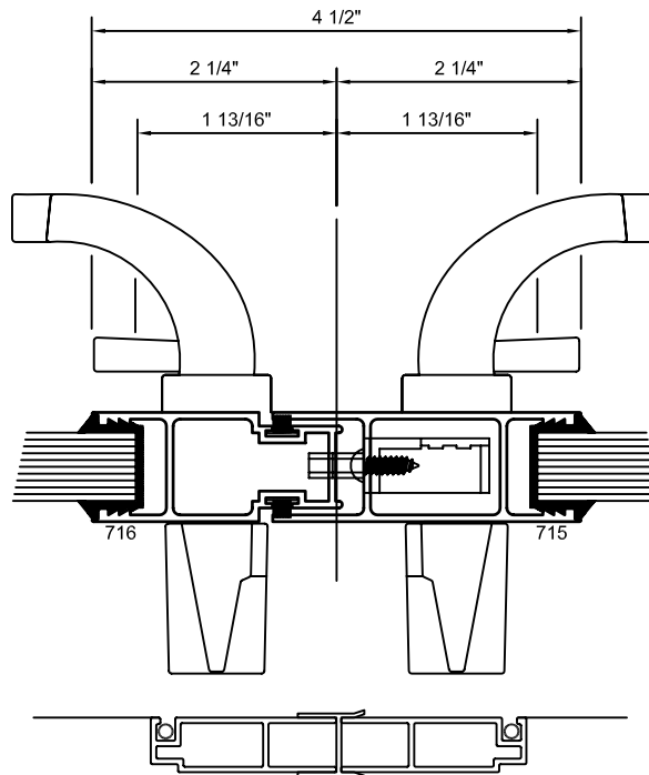
OXO LOCKING RAIL XOO/OOX MEETING RAIL (OMIT HANDLE)
