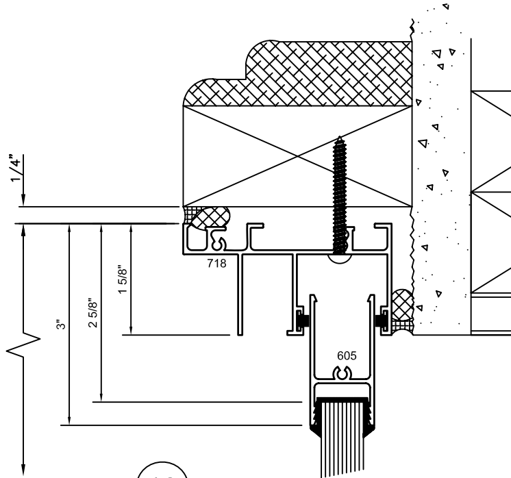
HEAD DETAIL POCKET DOOR
