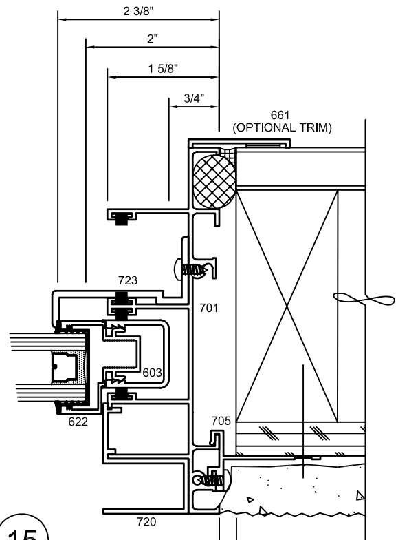
RIGHT JAMB (FIXED)
