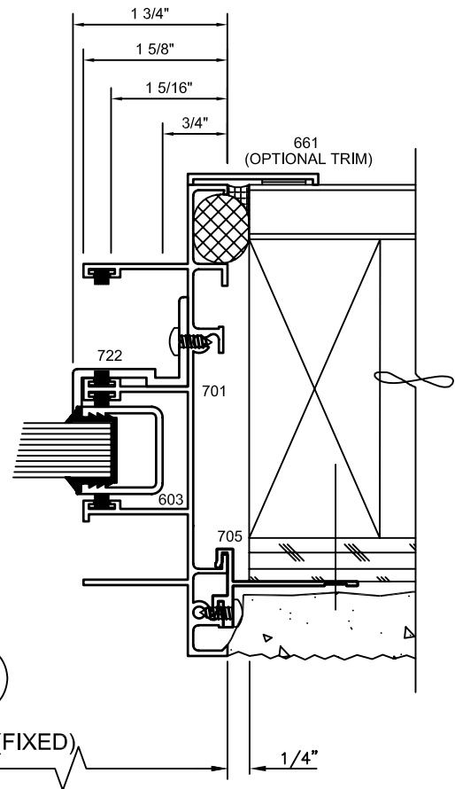
STANDARD INTERLOCK
