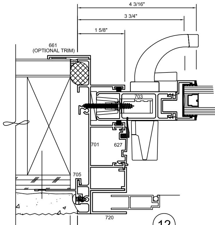
LEFT JAMB (OPERABLE)
