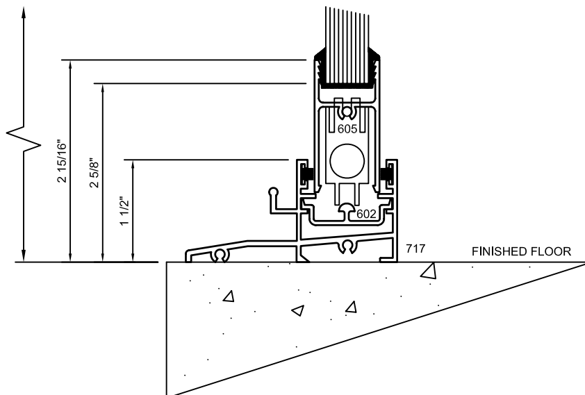
SILL DETAIL POCKET DOOR
